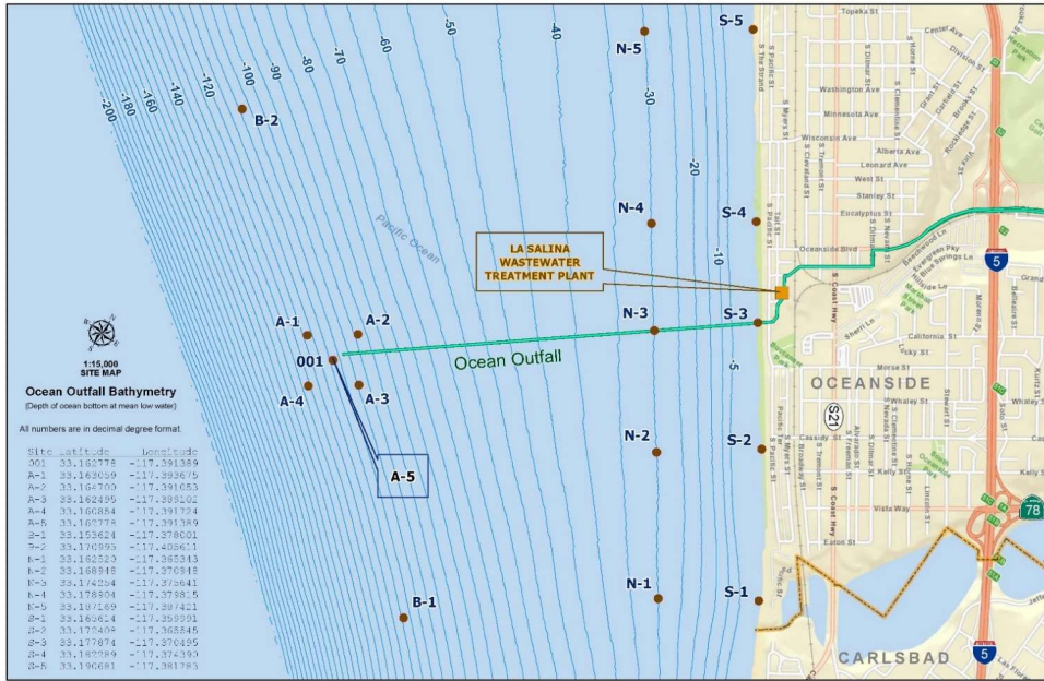
Oceanside Ocean Outfall Ocean Monitoring Locations
