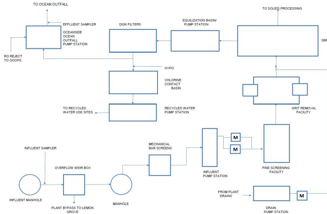
Process Schematic Southern Regional Tertiary Treatment Plant
