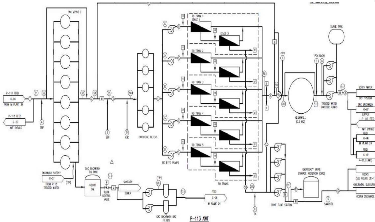
Process Schematic Advanced Water Treatment Plant at Haybarn Canyon
